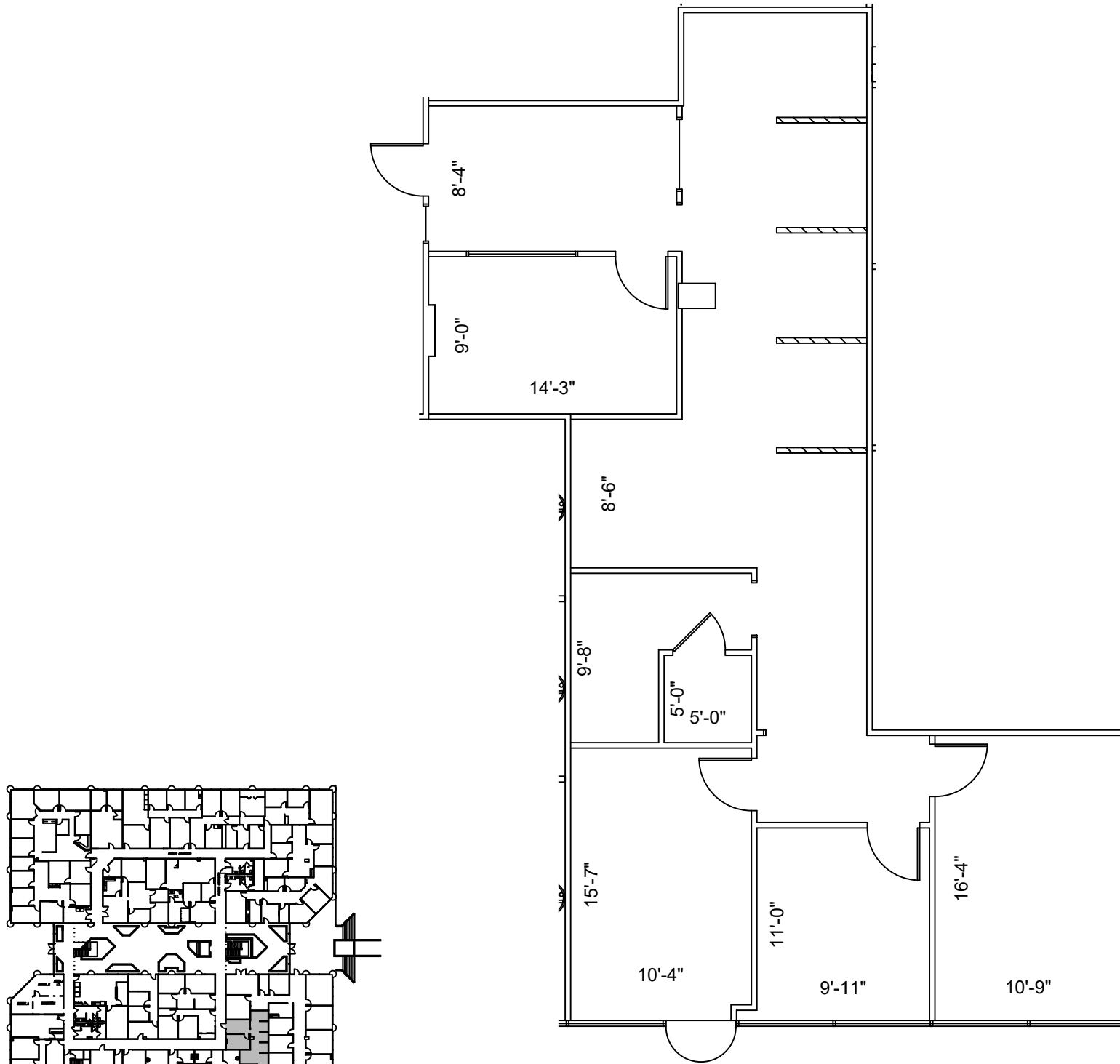
2nd FLOOR KEY PLAN
